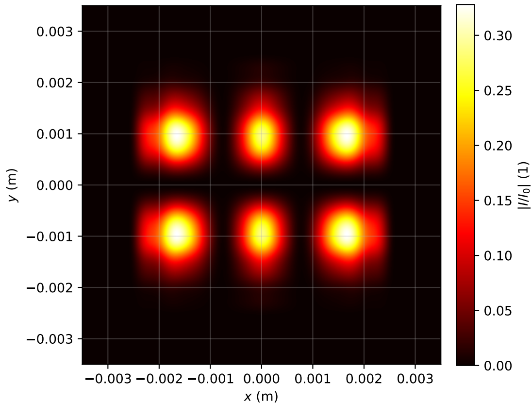
Intensity profile I(x, y, z = 3.662)/I_0 , P_{in}=2.0P_{cr} , artificial time
